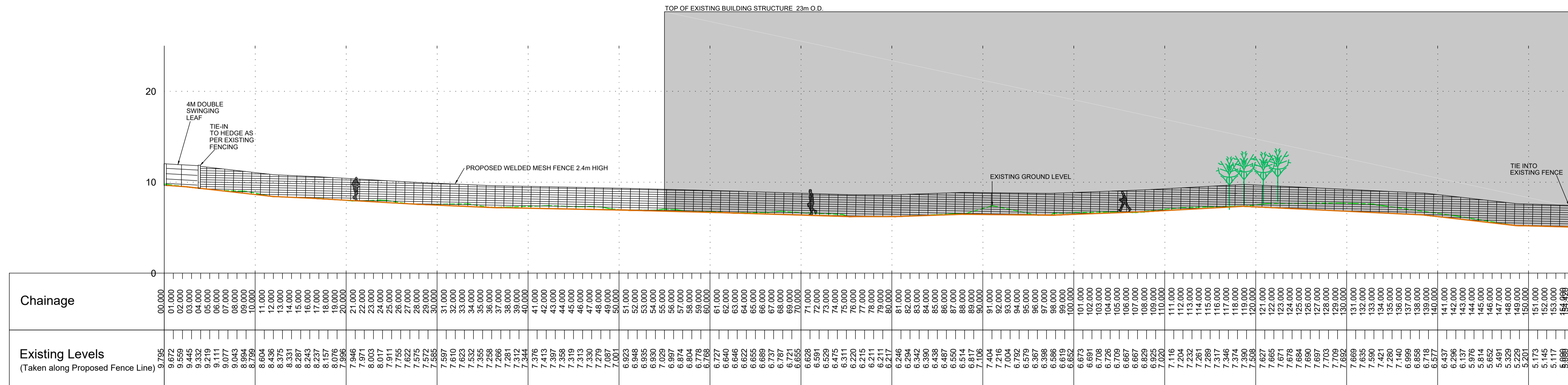
ALIGNMENT - LONGSECTION SCALE: H 1:250, V 1:250. DATUM: 0.000
